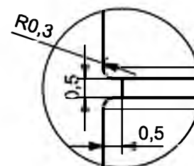
DETAIL B SCALE 10:1
