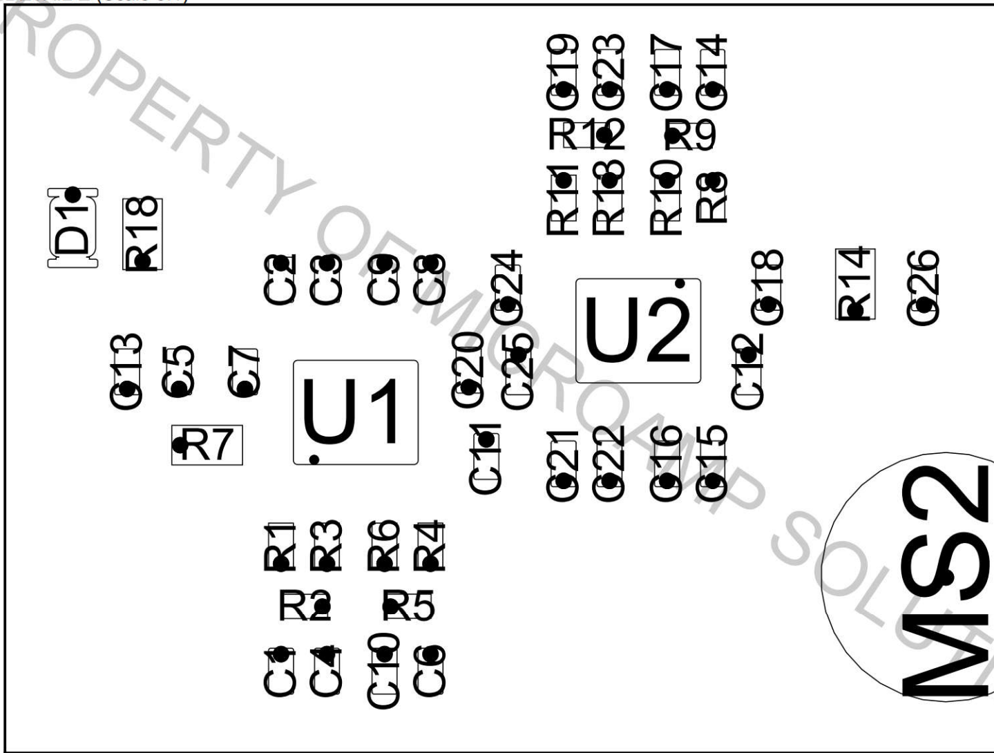
DETAIL E (Scale 8:1)
