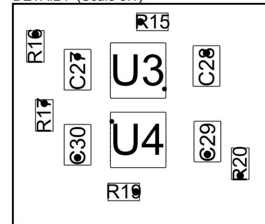
DETAIL F (Scale 5:1)
