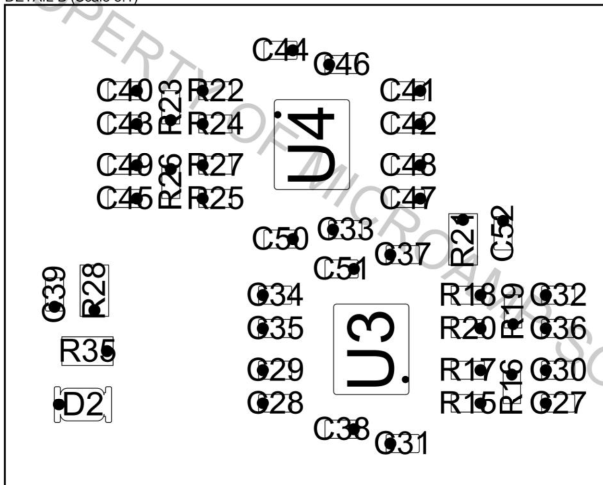
DETAIL B (Scale 8:1)
